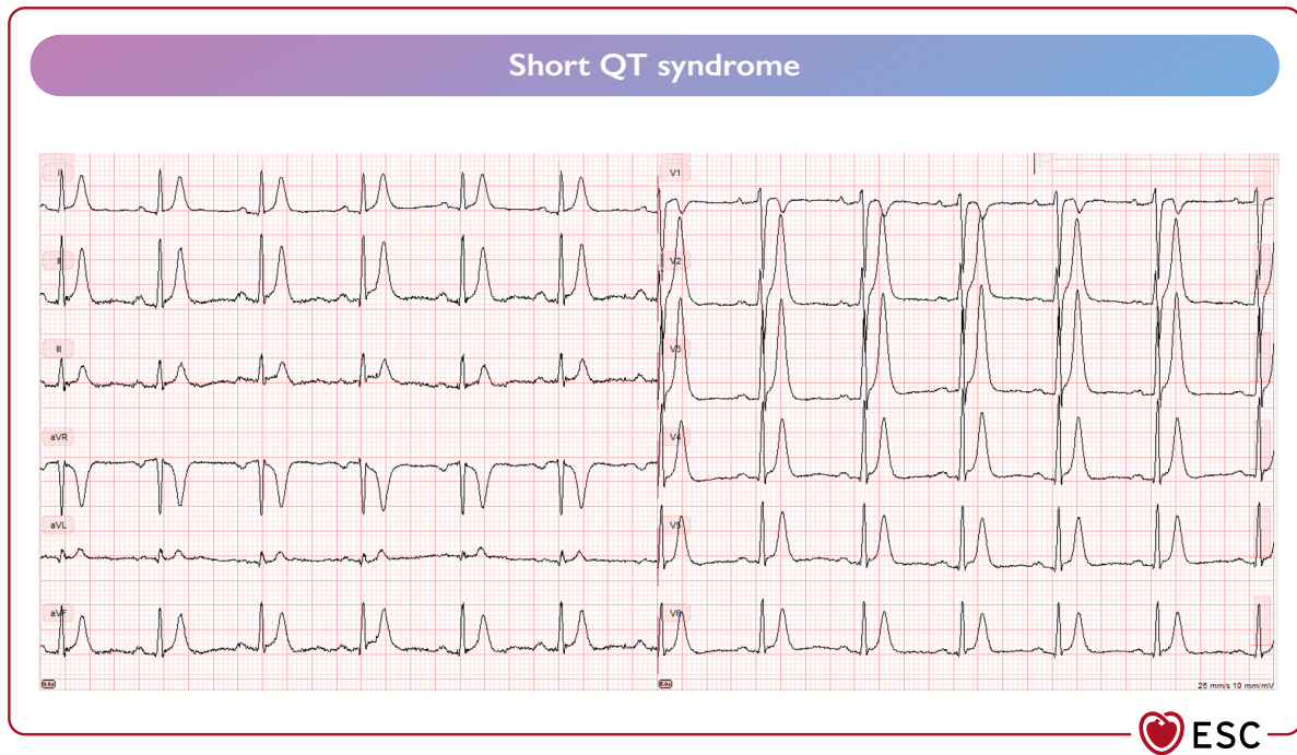
Figure 37 Short QT syndrome.
